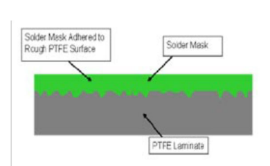
Figure 4 - Illustration of soldermask wetting and adhesion to rough PTFE surface
